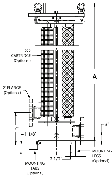
SWING BOLT STYLE
