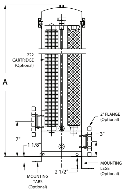
CLAMP STYLE
